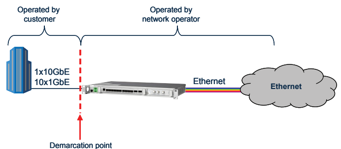
Fig 1. 10G Ethernet Access Solution providing Ethernet services
