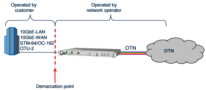
Fig 2. 10G OTN Access Solution providing optical services
