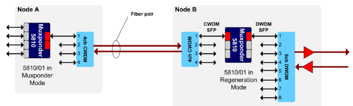
Fig. 2 CWDM to DWDM transition example
