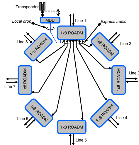
Fig. 2 2-dimensional node. Full connections only shown for Line 1
