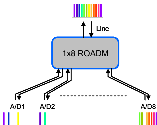
Fig. 1 Schematic principle of 1x8 ROADM add-drop function
