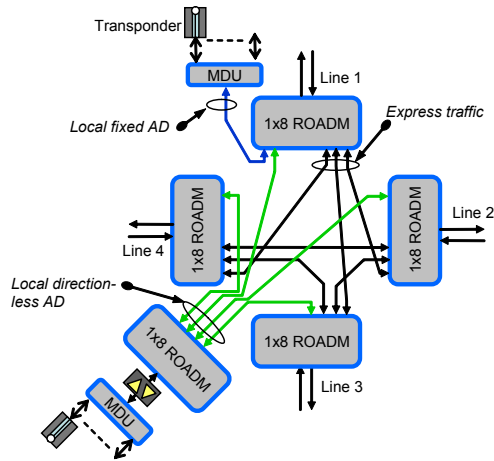
Fig. 3 A 4-dimensional node with both fixed and directionless traffic
